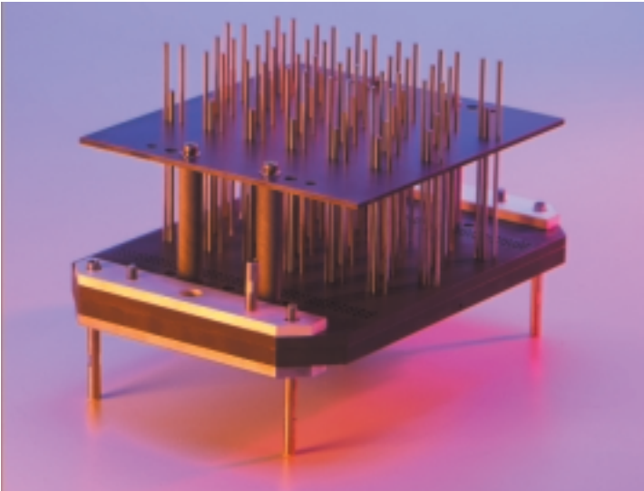
Graphite Fixture with Integrated Positioning Springs
